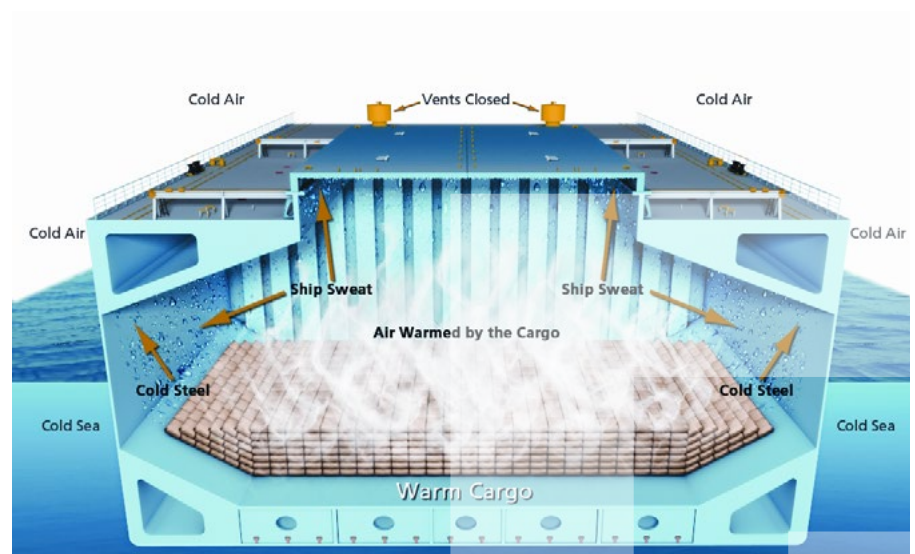
The Formation of Ship Sweat
